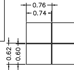
DOTS Detail Scale 10:1
